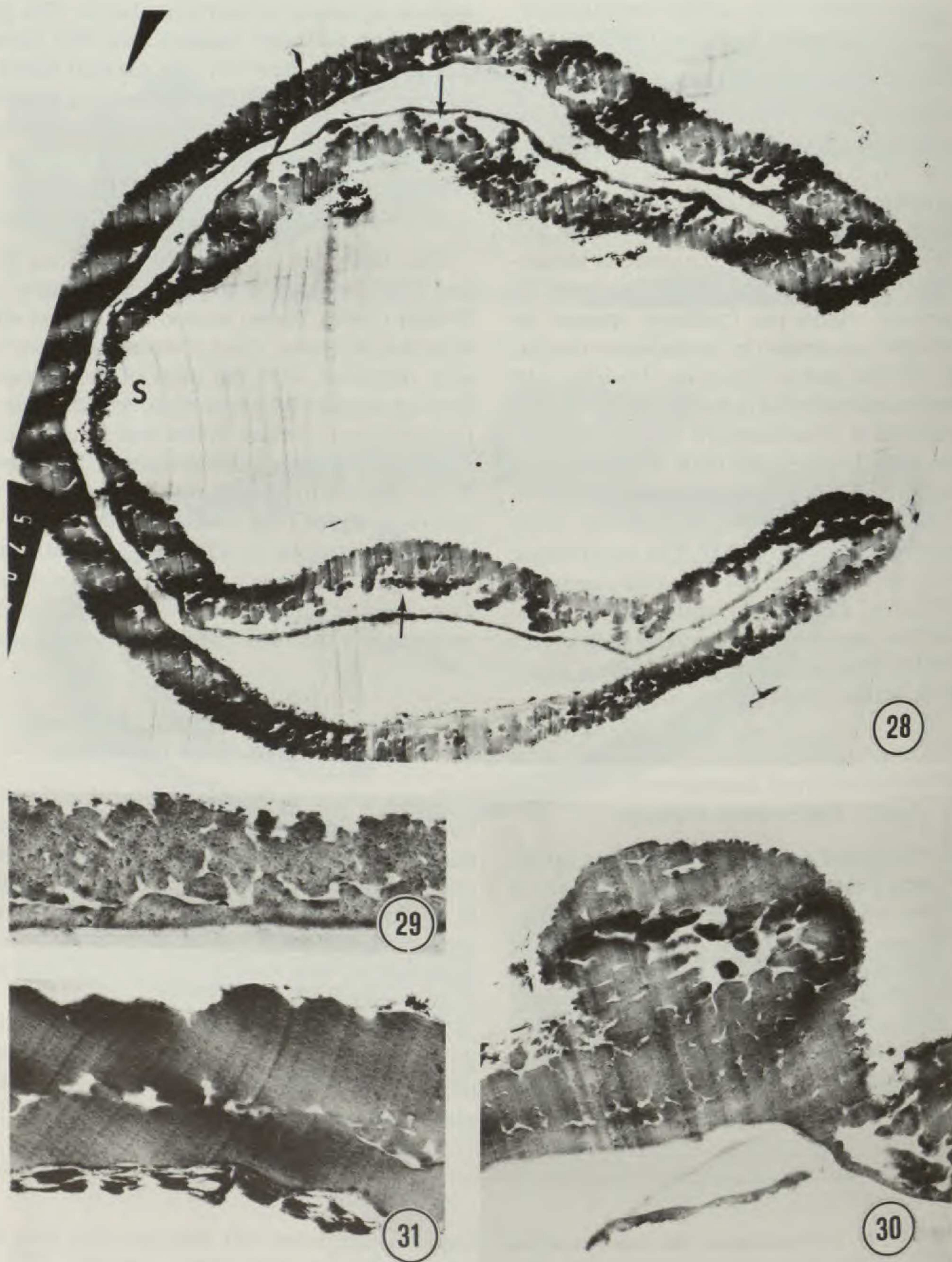
FIGURES 28-31. Transmission electron micrograph of fossil saccate pollen.—28. Transmission electron micrograph of vestigial saccate pollen grain (same grain pictured in Fig. 16), showing sulcus, separation of the footlayer (nexine 1), and outer wall layers (arrows) resulting in the sac and the granular infrastructure, \times 7,000 .—29. Punctamultivesiculites inchoatus , same grain pictured in Figure 15, transmission electron micrograph showing details of the wall structure; a thin inner non-lamellated footlayer (nexine 1), granular infrastructure, and outer tectum with suprategal scabrae, \times 14,200 .—30. P. inchoatus , same grain pictured in Figures 15 and 29, transmission electron micrograph showing wall structure of the pustule-like sacci, note it is not a simple separation of the footlayer and the outer layers of the exine, but is constructed of exinal material, \times 11,600 .—31. Verrumonocolpites conspicuus , same grain is pictured in Figure 18, transmission electron micrograph showing wall structure; thick footlayer (nexine 1), which is underlain by a thin, ragged lamellated layer (possibly endexine), granular infrastructural layer and thick tectum, \times 29,000 .
